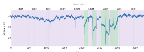
Fig. 1. Example output from AD of RxMER data with identified anomalies; the standing wave is highlighted across almost the full range of data, and multiple wireless ingresses are highlighted in green color on the right side of the figure.
