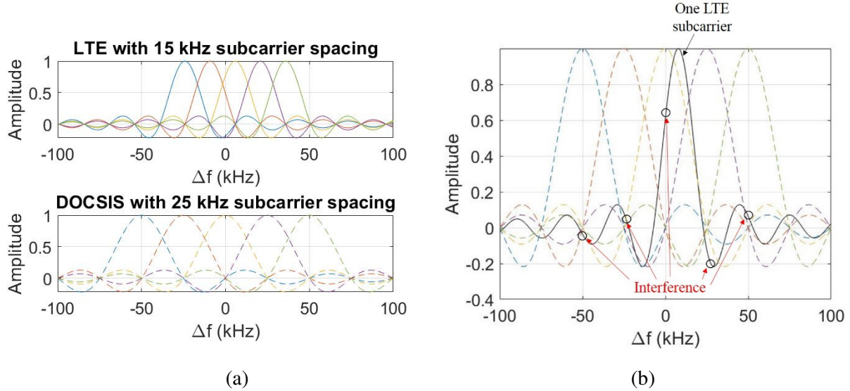
Figure 1. 25-kHz DOCSIS subcarrier spacing with random start frequency.
