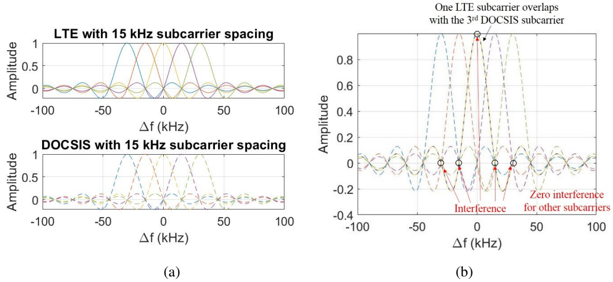
Figure 3. 15-kHz DOCSIS subcarrier spacing with frequency synchronization.
