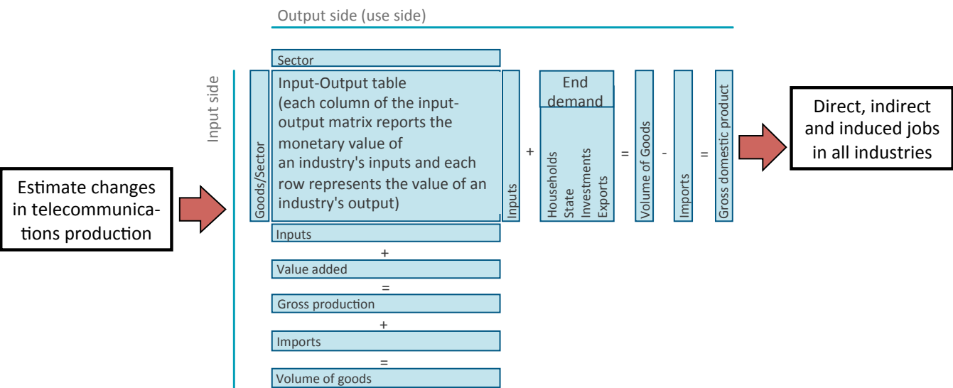
Figure C-1 Structure of an Input-Output Matrix
